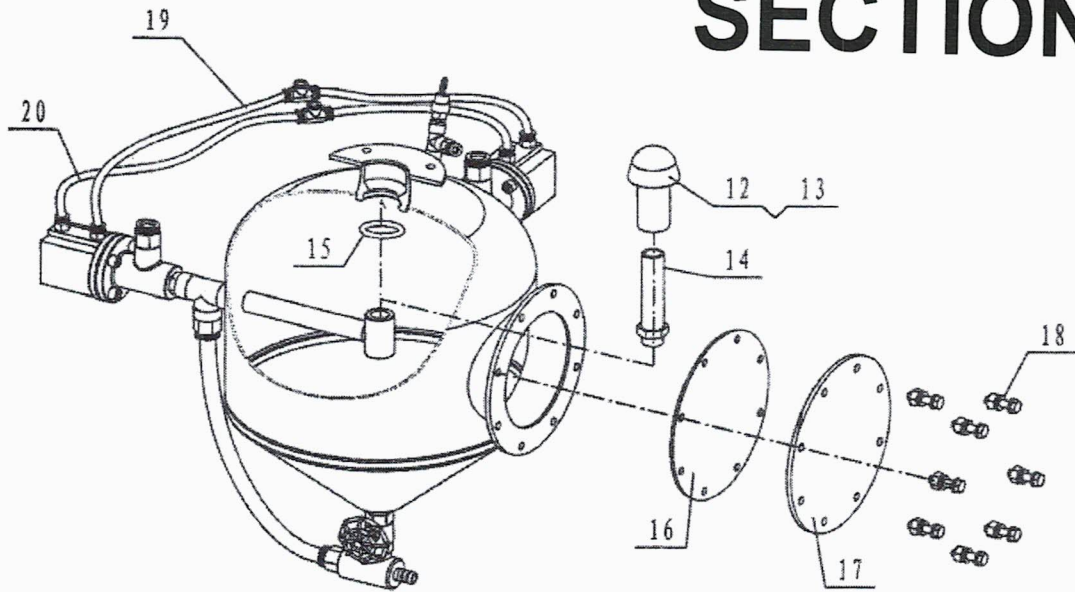
Exploded View of Tank Assembly
