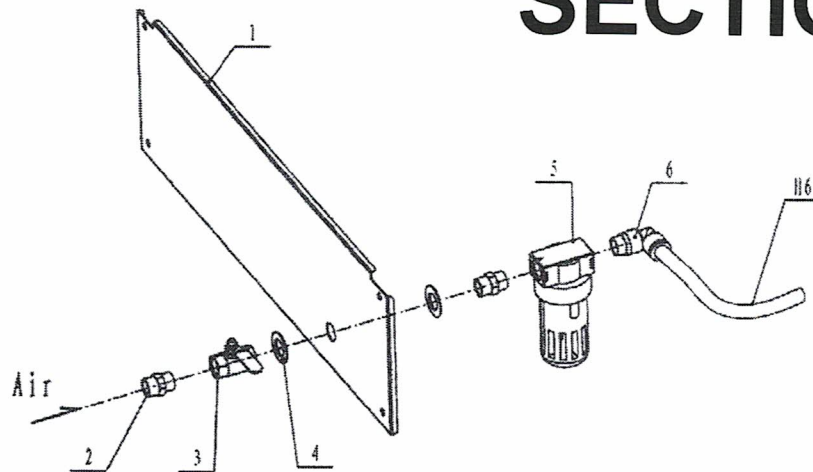
Exploded View Of Left Bar
