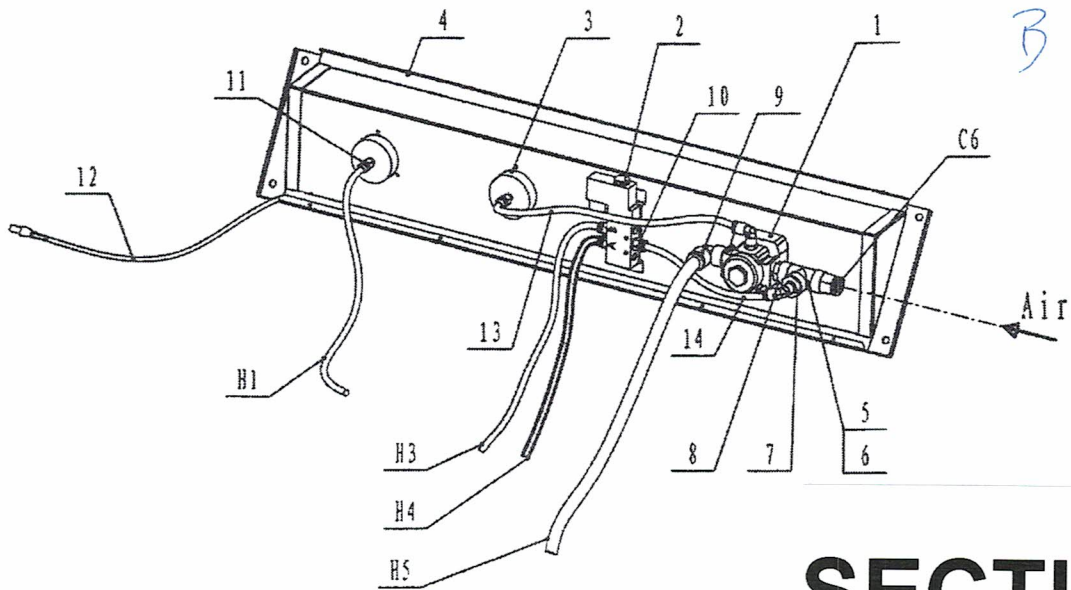
Exploded View of Control Panel
